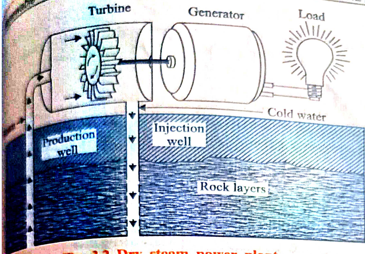
Fig. 3.2 Dry steam power plant
