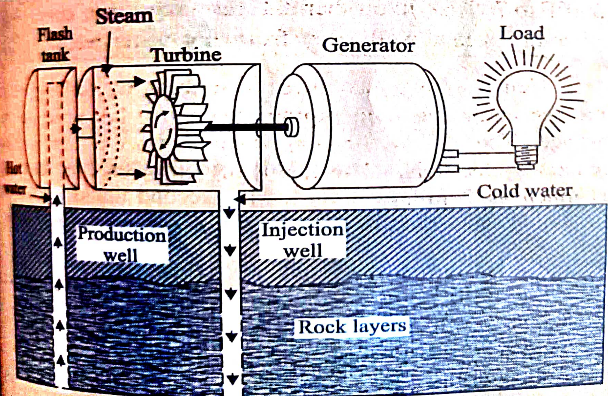
Fig. 3.3 Flash steam power plant
